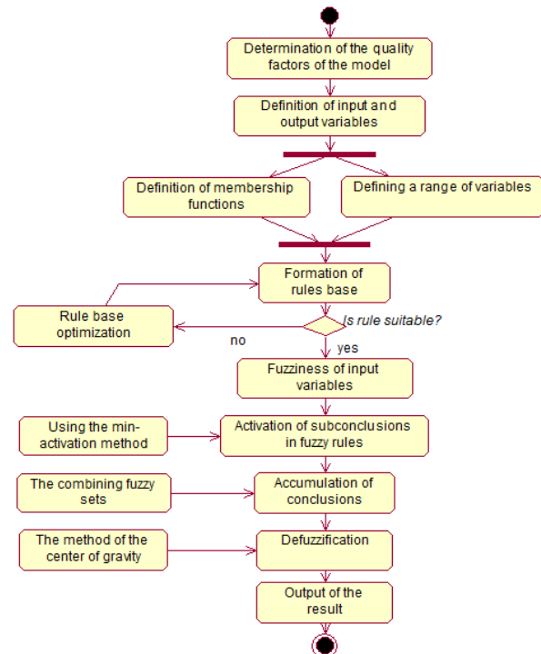
Fig. 1. The algorithm of functioning of the automated system
