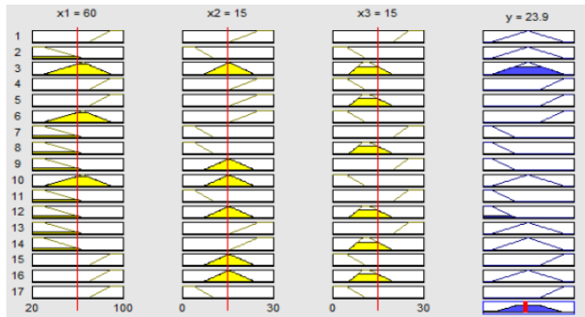
Fig.5. Output of results in Matlab
